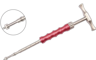
93310902-93004002 长尾万向钉上钉器(梅花) Long-arm multi-axial pedicle screw screwdriver,T3.4
