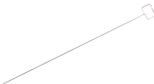
92215201 清洁导针 Cleaning Guide Pin , \Phi 2.0mm
