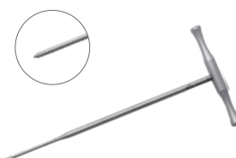
91162504 锁定丝锥 Tap, Ø2.5mm
