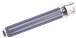
92101002 保护套筒 Protective Sleeve, \Phi 12.8 \times 125\text{mm}
